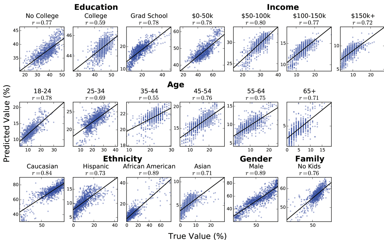
Figure 3: Scatter plots of the true demographic variables from Quantcast versus those predicted from the neighbor vector, along with the held-out correlation coefficient ( r ).
