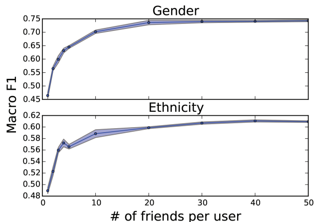
Figure 6: Macro F1 as the number of friends per user increases (with standard errors).
