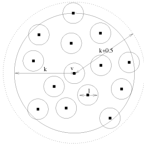
Fig. 2. For every node v , the number of dominators within k units is bounded by a constant \ell_k .
