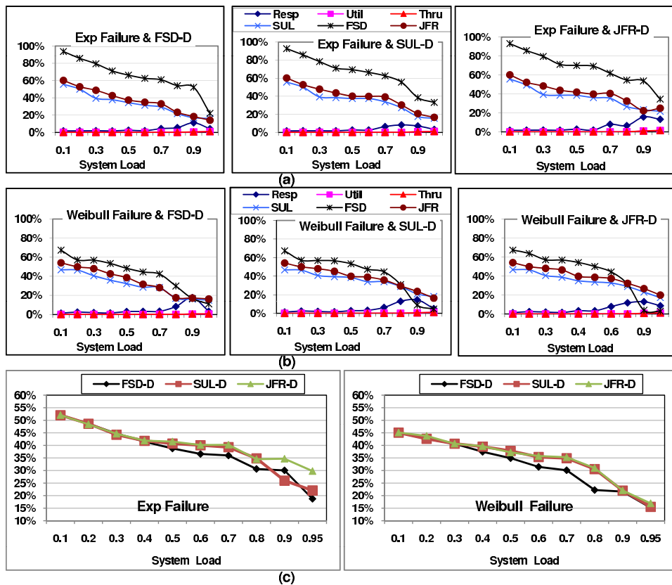
Fig. 6. Sensitivity to system load. Figure (a)-(b) plot the relative gain of each metric over FCFS, under Exponential Distribution and Weibull Distribution respectively. Figure (c) presents the overall gains of different rescheduling strategies, based on Kiviat graph. The performance of FARS drops as system load increases. FARS always outperforms FCFS by over 15%, even when the system has high load.
