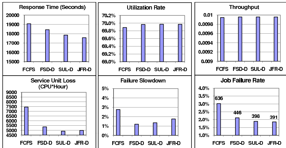
Fig. 5. Synthetic data under Weibull bathtub failure distribution. The data label in the plot of job failure rate indicates the actual number of failed jobs. The composite gain over FCFS, based on the Kiviat graph, is 33.73% (FSD-D), 36.62% (SUL-D), and 33.84% (JFR-D).
