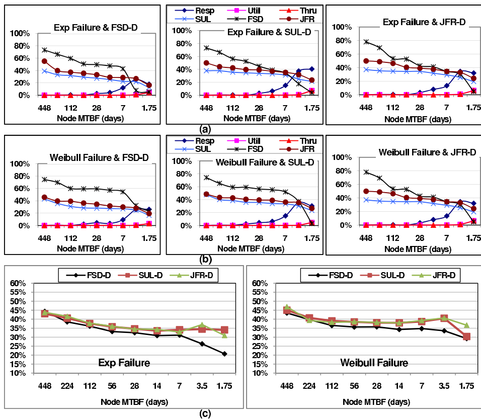
Fig. 7. Sensitivity to Node MTBF. Figure (a)-(b) plot the relative gain of each metric over FCFS under Exponential and Weibull failures respectively. Figure (c) presents the overall gains of different rescheduling strategies, where the overall gain is calculated based on Kiviat graph. The results show that in general, the benefit brought by FARS drops as node MTBF decreases.
