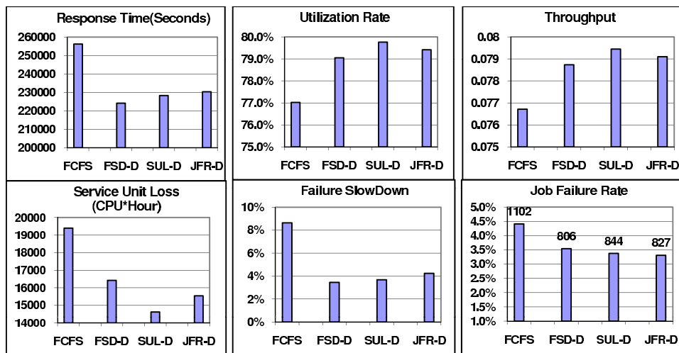
Fig. 9. Results on system traces. The data label in the plot of job failure rate indicates the actual number of failed job. The relative gain over FCFS, based on the Kiviat graph, is 35.45%(FSD-D), 38.47% (SUL-D), and 35.21% (JFR-D).
