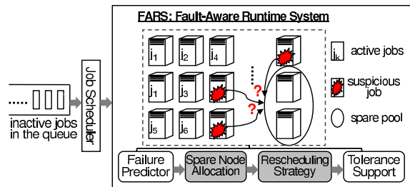
Fig. 1. Overview of FARS. User jobs are submitted through the job scheduler, while FARS is responsible for managing active jobs (i.e. running jobs) in the presence of failure. The dark shaded boxes indicate the major contributions of this study: spare node allocation (Section III) and job rescheduling (Section IV)
