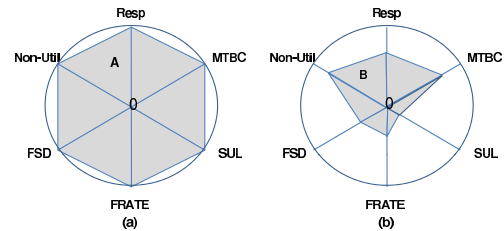
Fig. 3. Exemplar 6-D Kiviati Graph. The range of each metric is from zero to the largest value observed in the experiments. The relative gain of method B over A is defined as \frac{K(B) - K(A)}{K(A)} , where K(\cdot) denotes the K-value of a method. The K-Value of a method is the shaded area. The smaller a K-value is, the better performance a method has.
