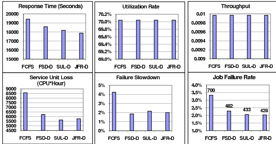
Fig. 4. Synthetic data under Exponential failure distribution. The data label in the plot of job failure rate indicates the actual number of failed jobs. The composite gain over FCFS is 34.02% (FSD-D), 36.35% (SUL-D), and 37.34% (JFR-D).
