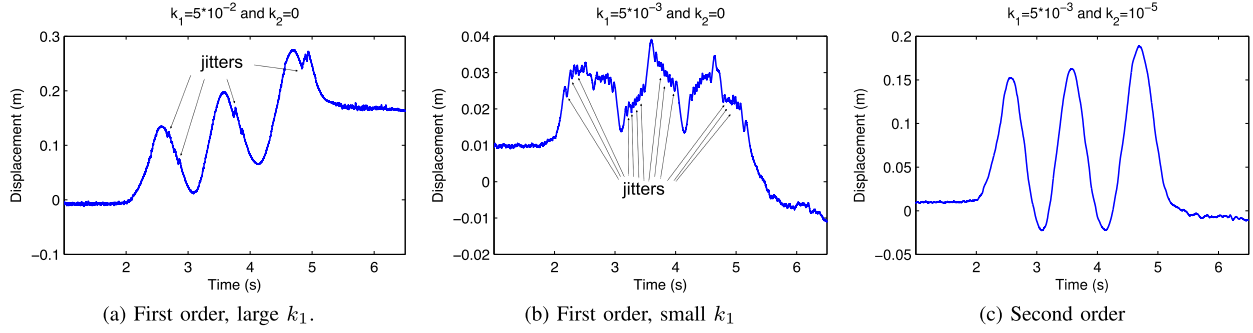
Fig. 7. Calculated displacement by PLL with different orders and parameters, when the signal is weak.
