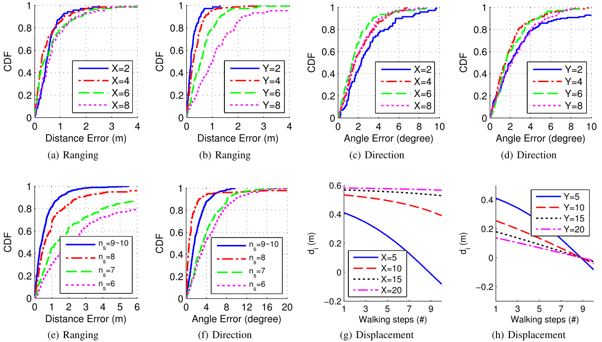
Fig. 12. The accuracy of ranging and direction finding. 1) when the user starts walking at different positions (a)(b)(c)(d), 2) when the user walks for smaller number of steps (e)(f). Relative displacements when users walks from different starting points.
