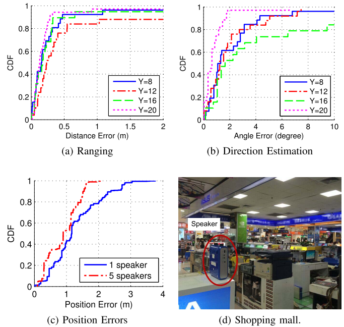
Fig. 15. (a), (b) Positioning after pulse detection. (c) Result of relative and absolute positioning. (d) The shopping mall and the dummy speaker.
