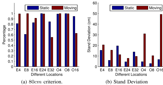
Fig. 14. (a) Percentage of successful experiments at different locations, (b) standard deviation.
