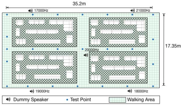
Fig. 16. The map of the shopping mall.
