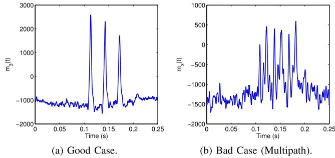
Fig. 10. Pulse detection in case of multipath effects.
