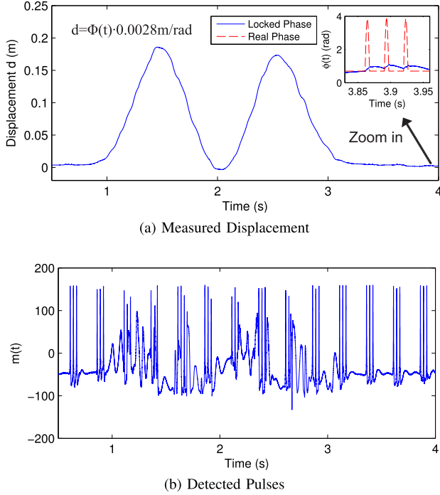
Fig. 8. Calculated displacement and pulses from the same signal.
