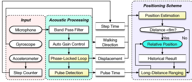
Fig. 2. The architecture of WalkieLokie.
