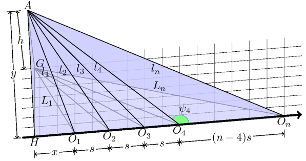
Fig. 3. Positioning when the user walks along a line.
