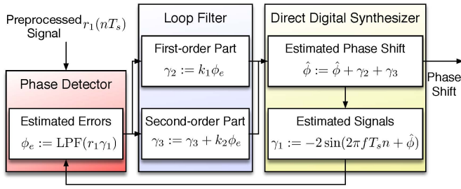
Fig. 6. Design of the second-order phase locked loop.
